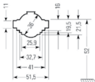
4NF03 400 A / 5 A a 800 A / 5 A
